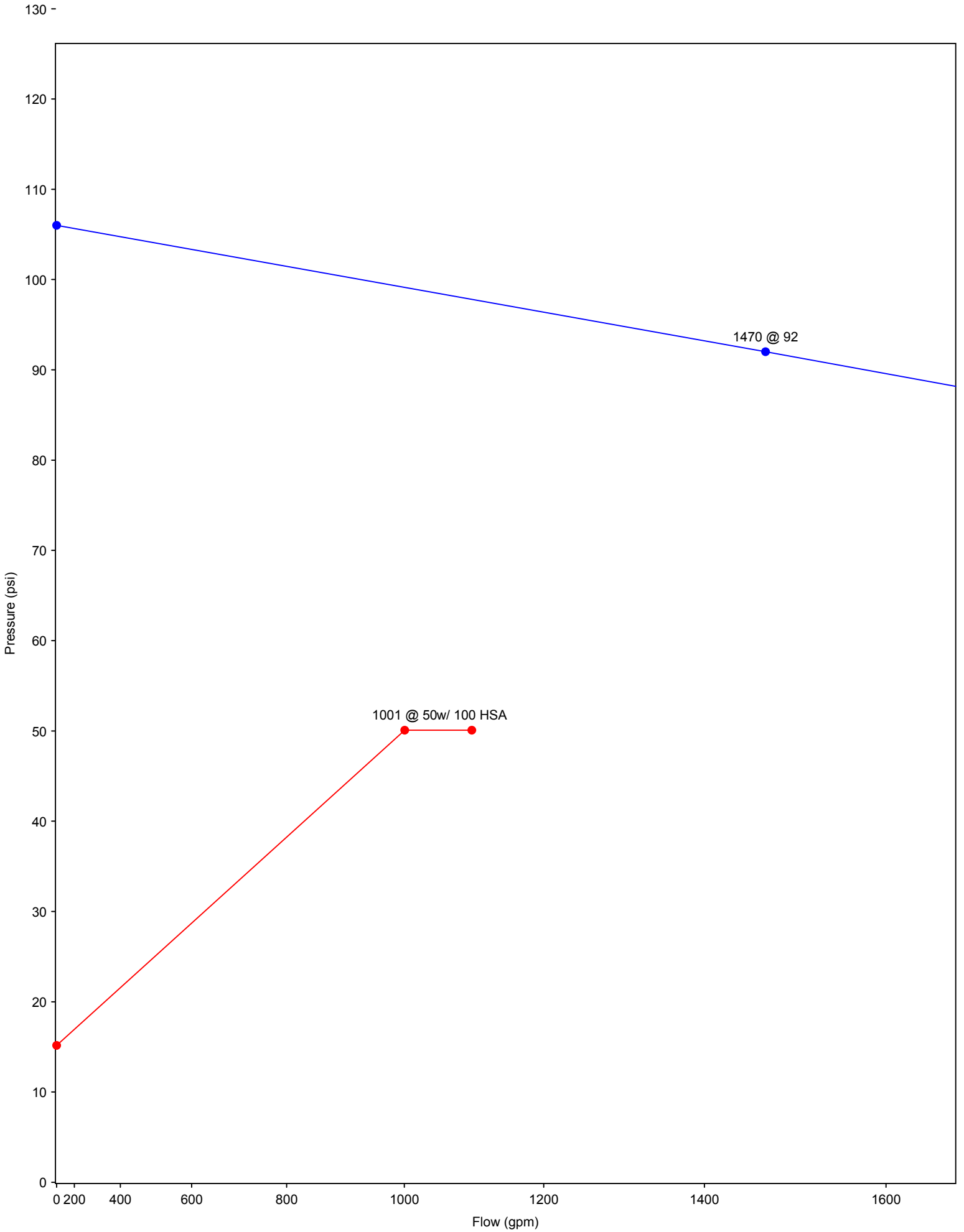
Water Supply vs. Sprinkler Demand
